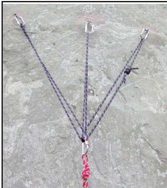
Figure 5-18. Self-equalizing anchors.
